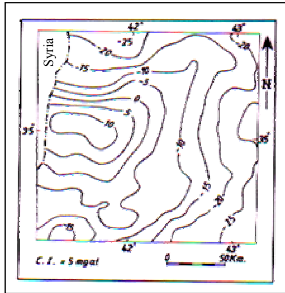
(Fig.2) Bouguer anomaly map of the studied area
