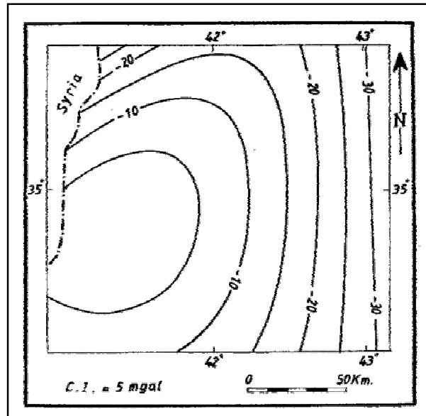
(Fig.6) Regional gravity map of the investigated area.
